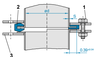
JACOB loose flange system
