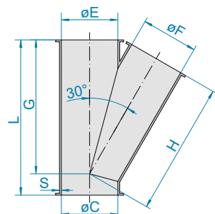
Lateral 30°
