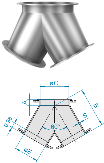
Stainless steel with galvanized loose flanges (dimensions for 14 gauge tubing)
