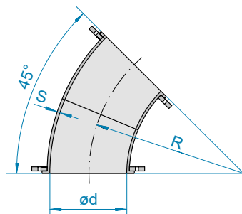
2 pressed segments 45°
