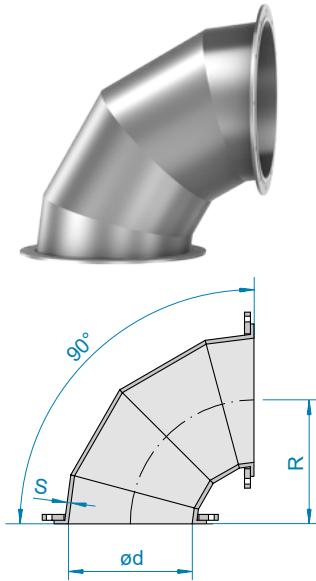
4 flat back segments: 2x30° / 2x15°
