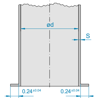
JACOB tubing system with a lip for pull ring connection
