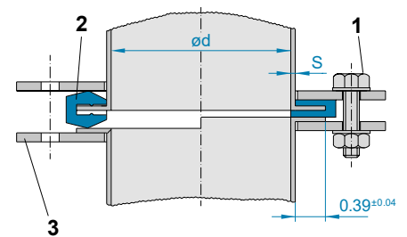
JACOB loose flange system
