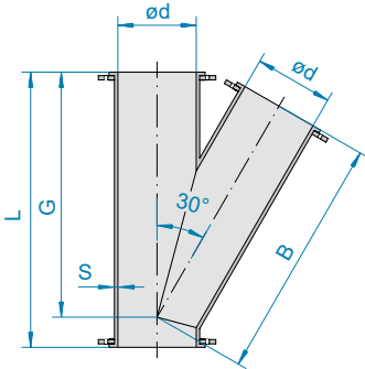
Lateral 30°
