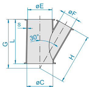
Conical lateral 30°
