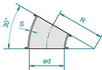
1 pressed segment 30°
