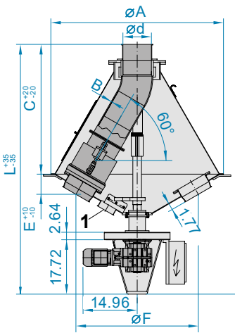
1 Drain nozzle
