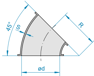
1 pressed segment 45°
