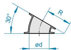
Cast-iron segment 30°
