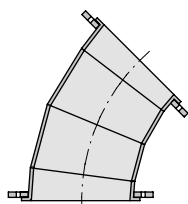
4 flat back segments: 2 x 15° / 2 x 7.5°
