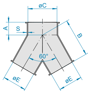
Conical Y-branch 60°
