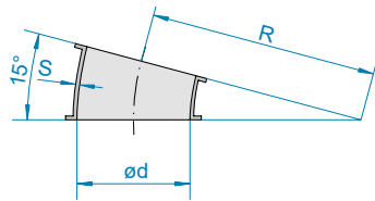
1 pressed segment 15°
