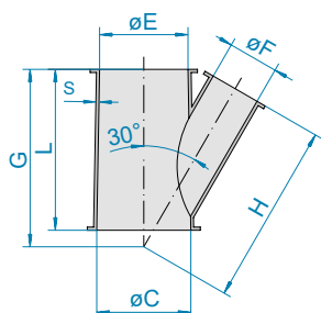
Conical lateral 30°
