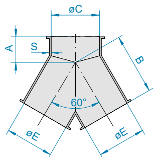
Y-branch 60°
