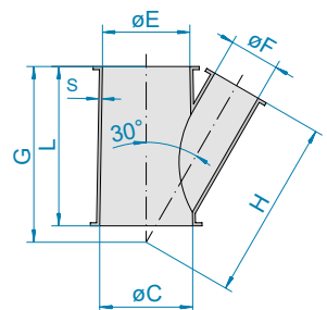
Conical lateral 30°
