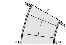
3 flat back segments: 1x15° / 2x7.5°
