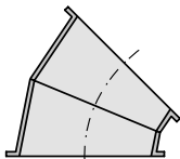
2 flat back segments: 2 x 22.5°
