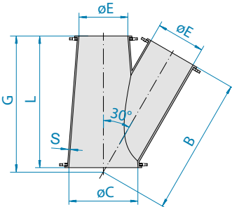
Conical lateral 30°
