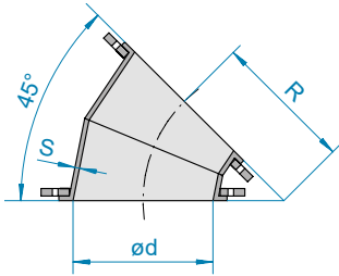
2 flat back segments 22.5°
