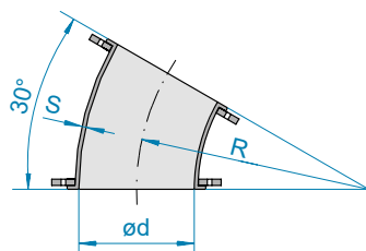
1 pressed bend 30°
