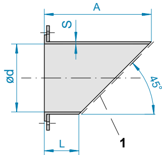
1 Bird-guard
