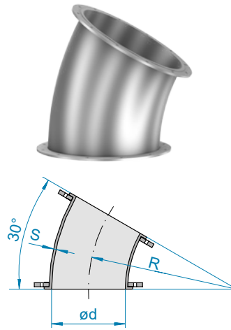
1 pressed bend 30°
